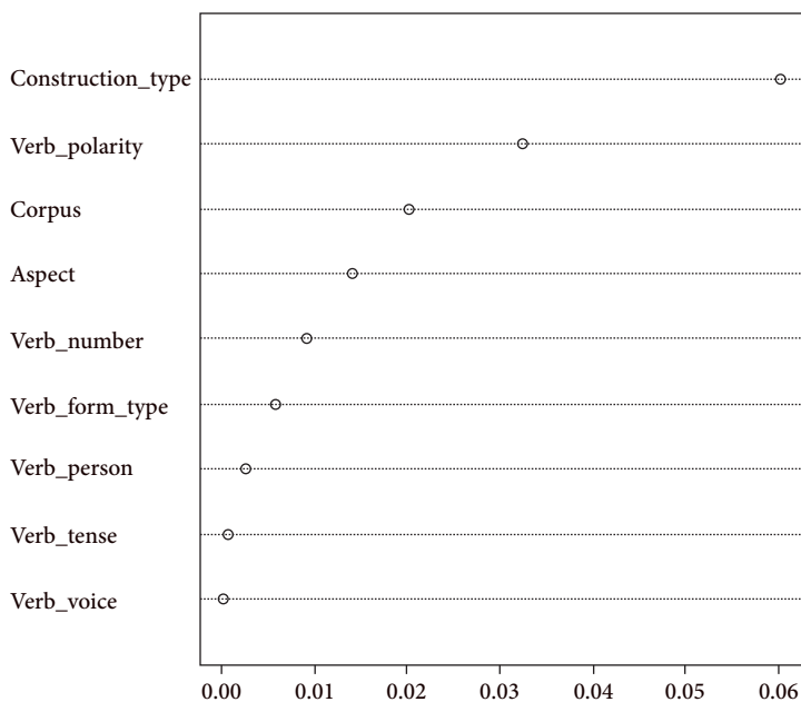
Figure 2. Variable importance plot
